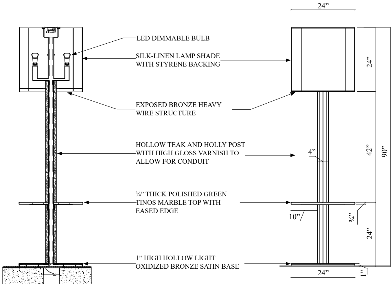
SECTION DETAIL
