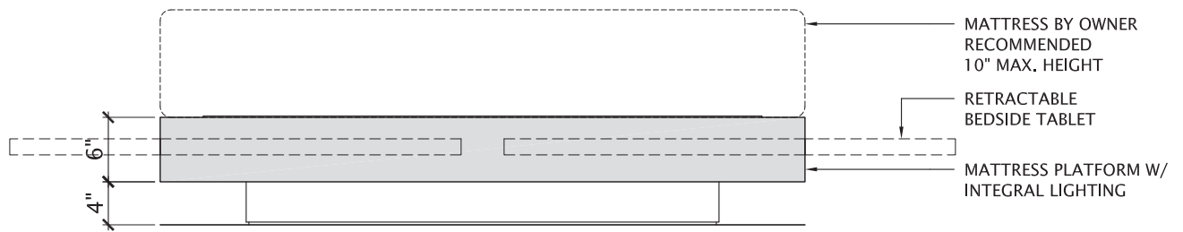
END ELEVATION QUEEN PLATFORM WITHOUT DRAWERS
