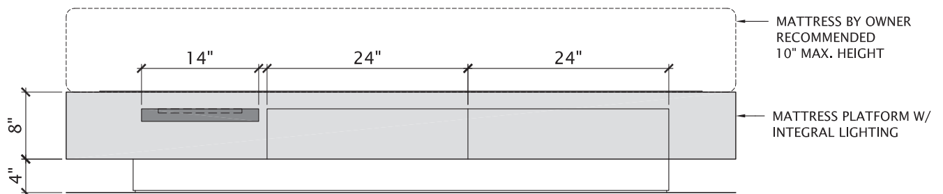
SIDE ELEVATION QUEEN PLATFORM WITH DRAWERS
