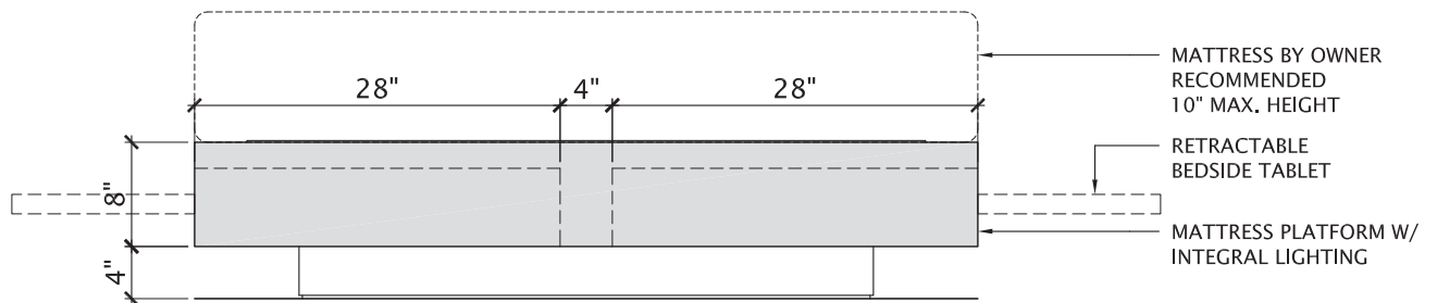
END ELEVATION QUEEN PLATFORM WITH DRAWERS
