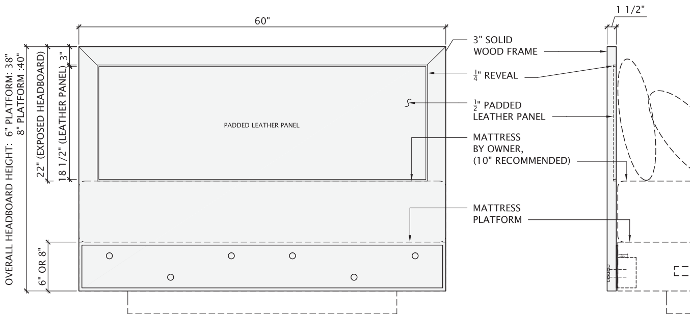
HEADBOARD ELEVATIONS FOR QUEEN PLATFORM WITH AND WITHOUT DRAWERS
