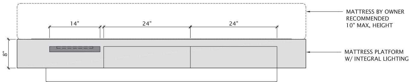
SIDE ELEVATION KING PLATFORM WITH DRAWERS
