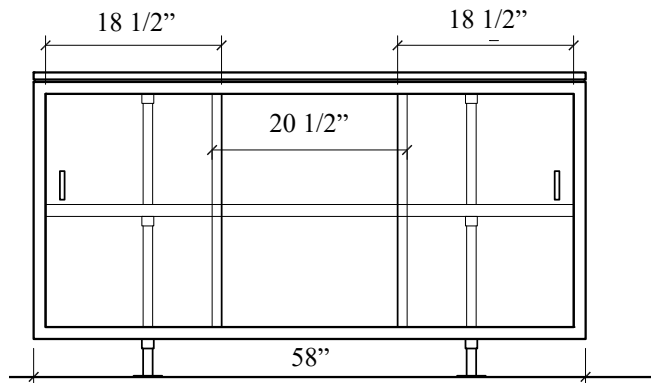
DISPLAY SIDE ELEVATION
