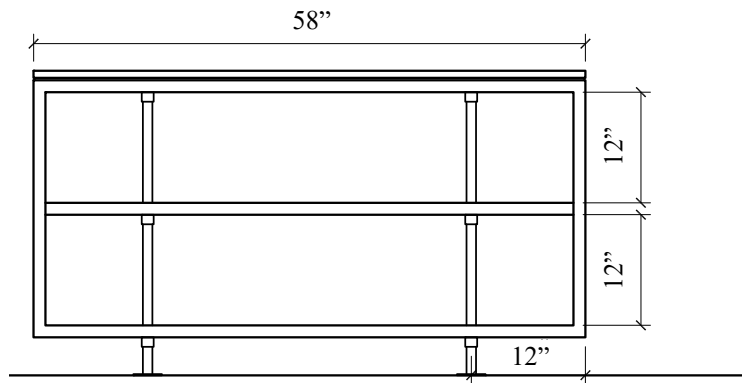
BOOKSHELF SIDE ELEVATION
